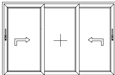
Schema C 2 ante mobili 1 fissa 3 binari 2 mobile sashes, 1 fix sash 3 tracks
