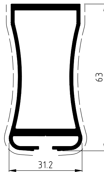
RINFORZO CENTRALE CENTRAL REINFORCED PROFILE
