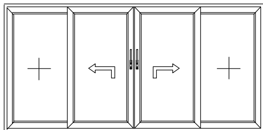
Schema E 2 ante mobili 2 ante fisse 2 binari 2 mobile sashes, 2 fix sashes 2 tracks
